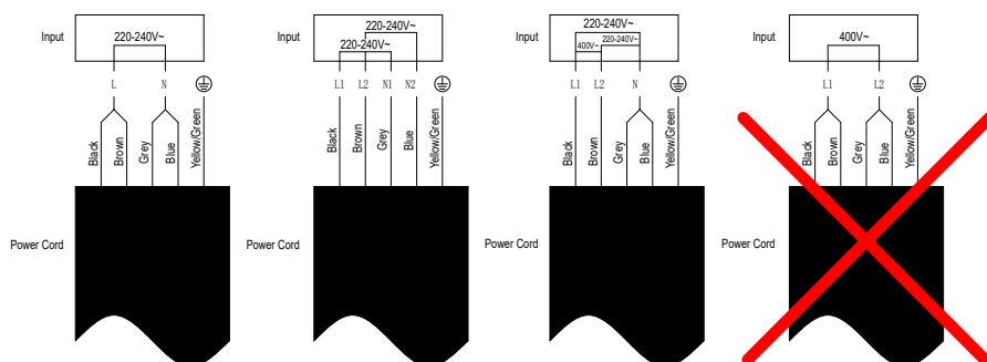
30cm 2 zones induction hob or ceramic hob wiring diagram
